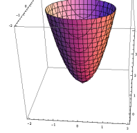
Paraboloide ax^2 + by^2 - z = 0
